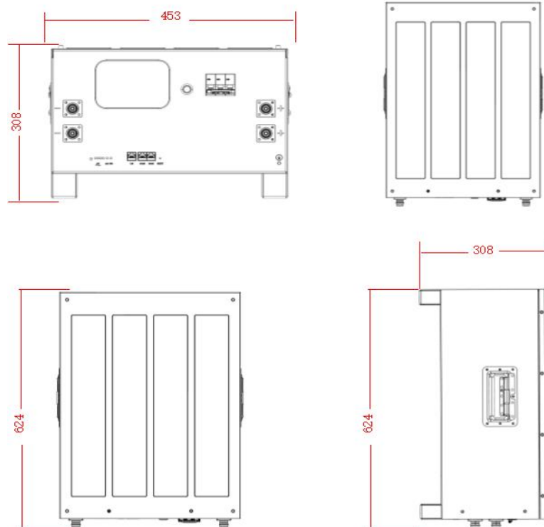
Battery module size diagram
